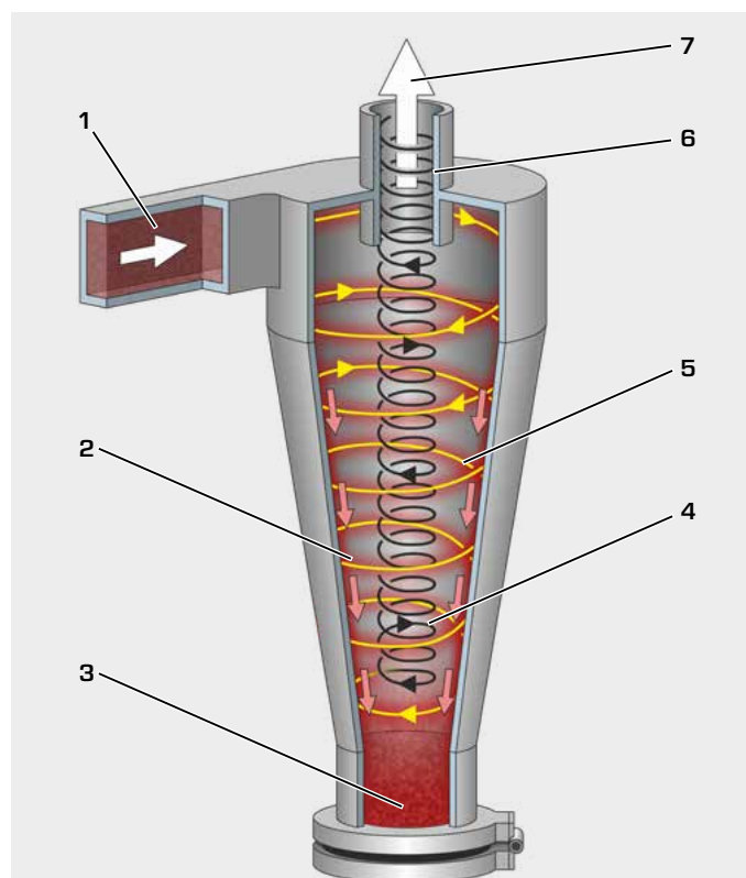
Gas cyclone:
