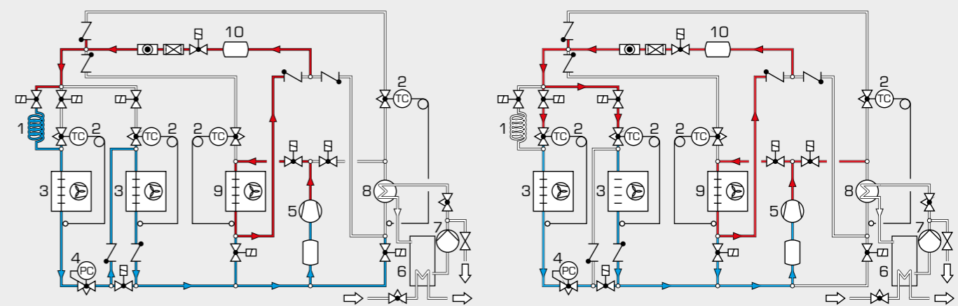
1 capillary tube, 2 expansion valve, 3 evaporator, 4 evaporation pressure controller, 5 compressor, 6 tank for glycol-water mixture, 7 pump, 8 coaxial coil heat exchanger, 9 heat exchanger with fan, 10 receiver
