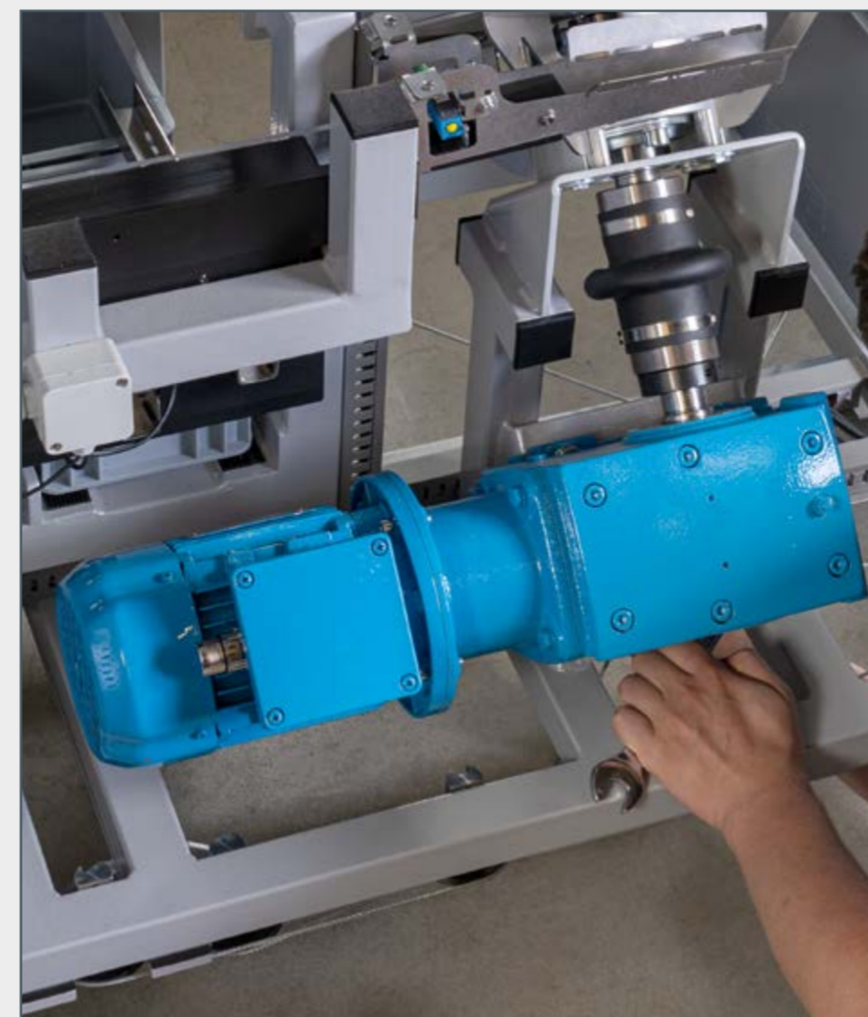
undo the threaded joint between the drive train and the frame in MT174
