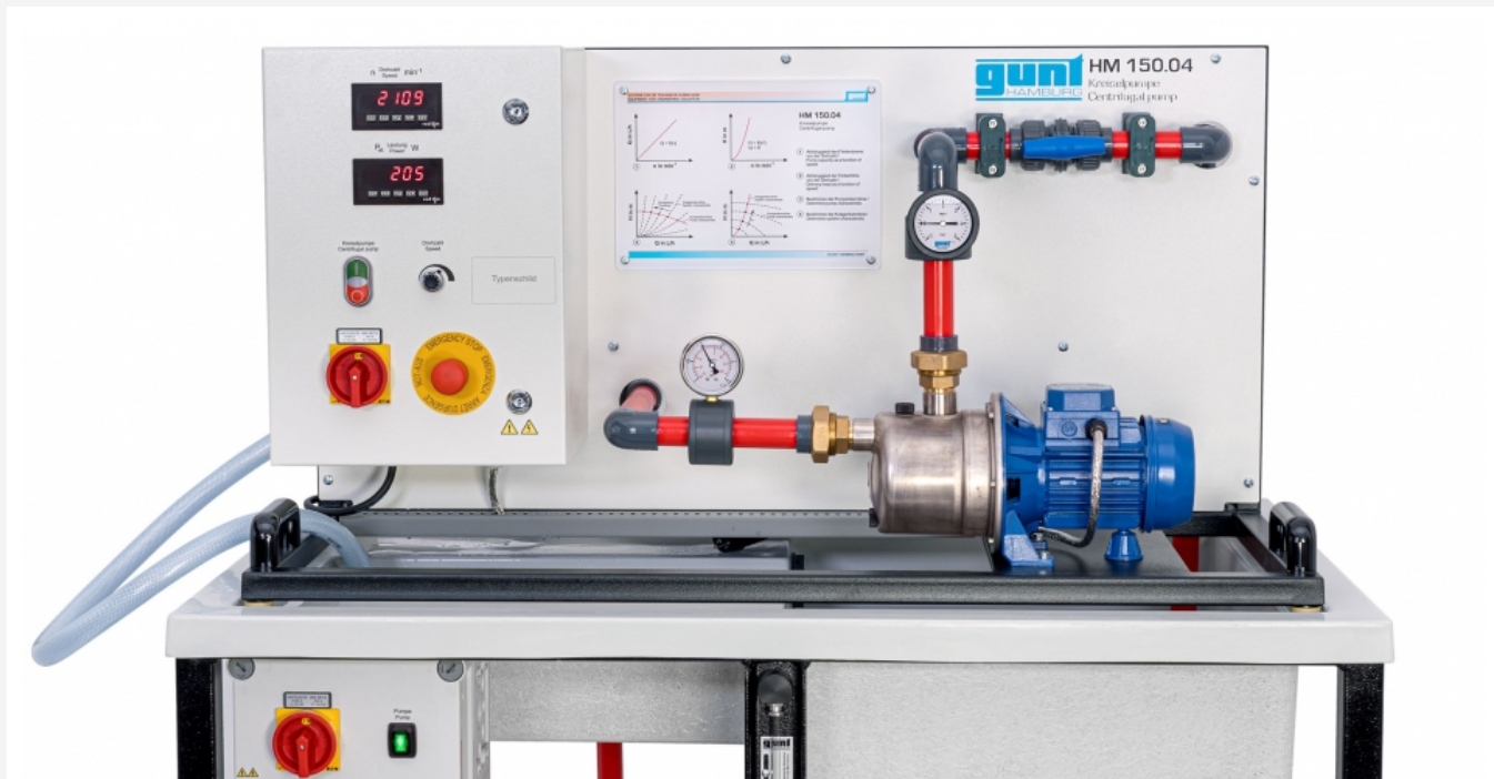
The illustration shows HM 150.04 together with HM 150.
